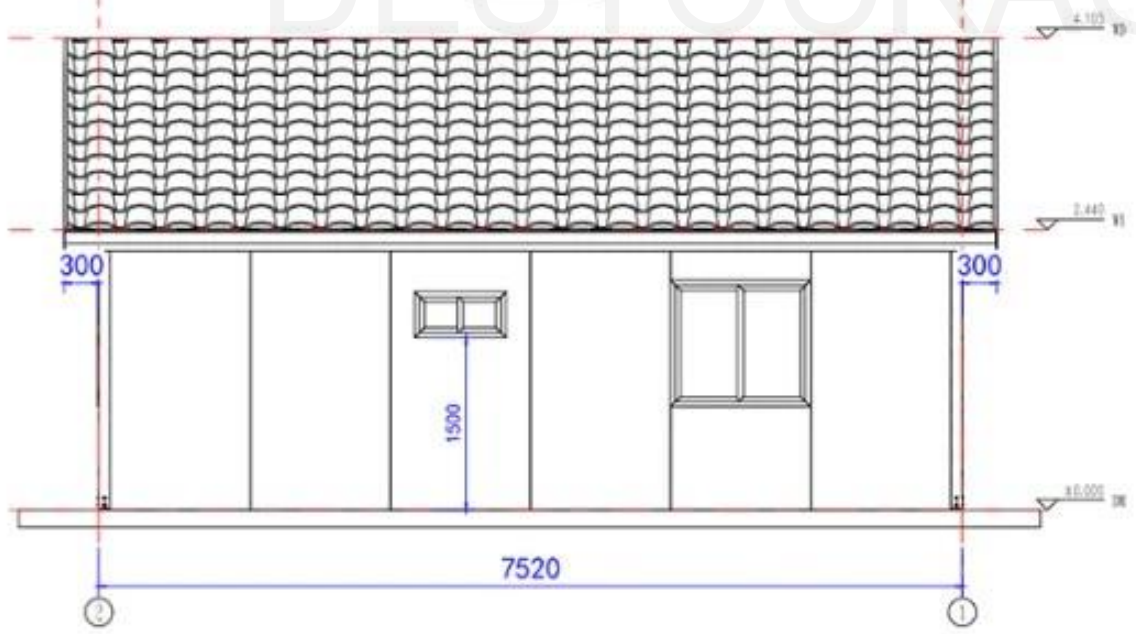
North view
